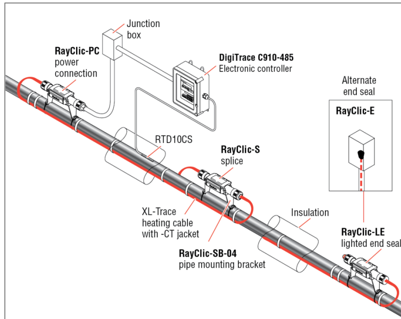
System for flow maintenance of above ground greasy waste disposal lines with line sensing control, monitoring, integrated ground-fault circuit protection and BMS communication capabilities.
