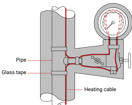
Figure 12: Pressure gauge
