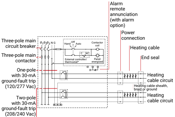
Figure 25: HTPG schematic
