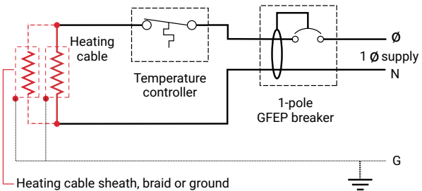
Figure 22: Single circuit control
