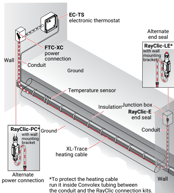
Figure 18: Buried pipe XL-Trace System
