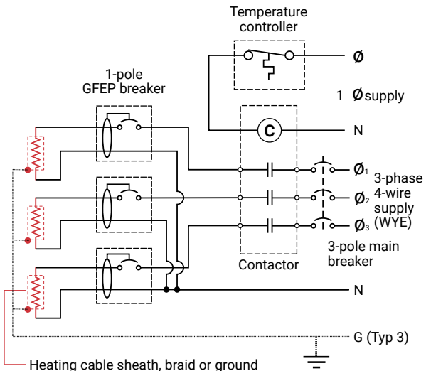
Figure 23: Group circuit control
