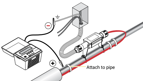
Figure 26: Insulation resistance test
