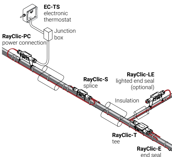
Figure 17: Aboveground nVent XL-Trace System
