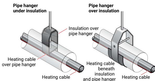
Figure 16: Pipe hanger
