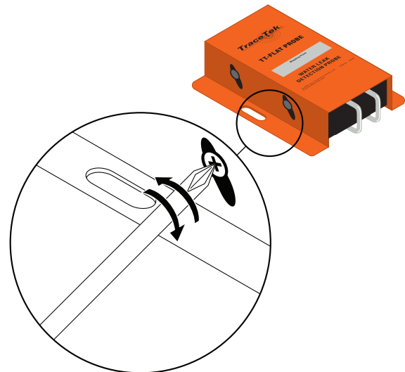
Figure 4. Adjusting the sensor tip height
