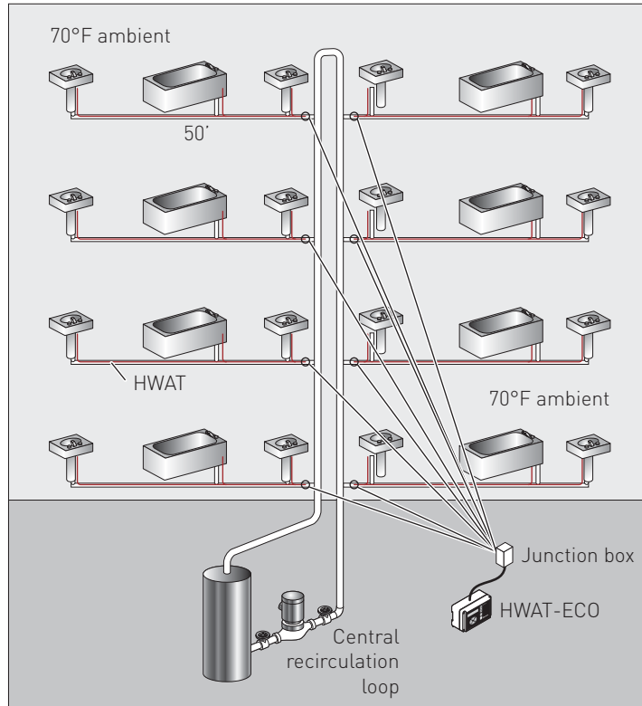
Fig. 1 Generic hybrid HWAT system
