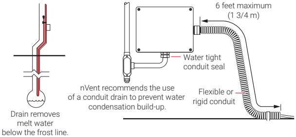
Figure 14: Installation of IceStop cable in trench drains
