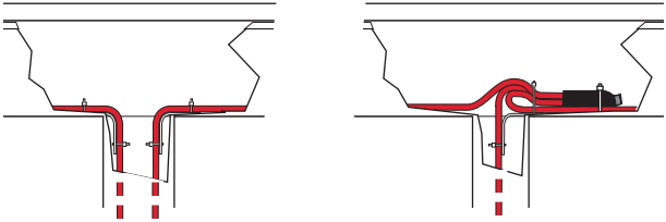
Figure 23: GM-RAKE downspout hangers
