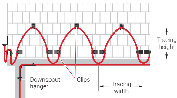
Figure 3: Front view of roof with IceStop system
