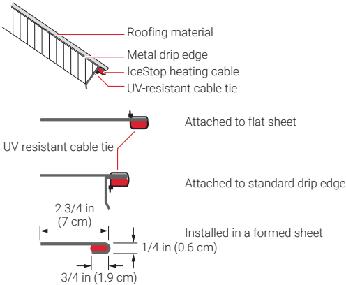
Figure 24: Heated drip edge attachment guidelines
