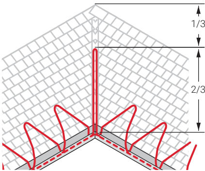
Figure 10: Layout for a roof valley
