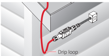
Figure 25: Drip loops
